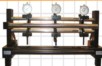
Shaft Gauging
