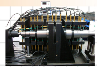
Main shaft
